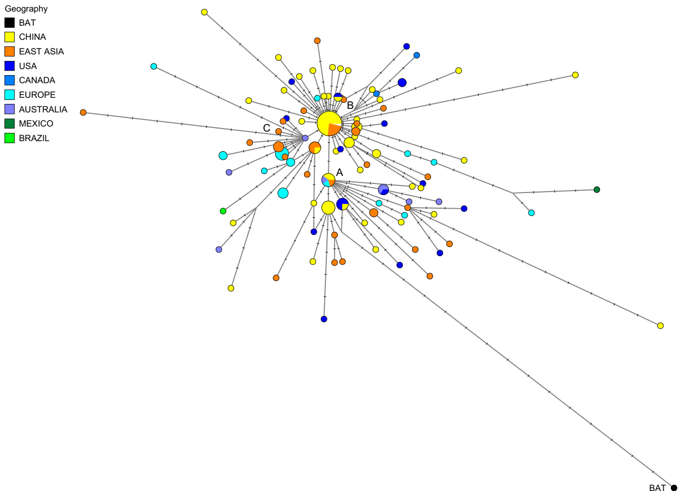
Fig. 1. Phylogenetic network of 160 SARS-CoV-2 genomes. Node A is the root cluster obtained with the bat ( R. affinis ) coronavirus isolate BatCoVraTG13 from Yunnan Province. Circle areas are proportional to the number of taxa, and each notch on the links represents a mutated nucleotide position. The sequence range under consideration is 56 to 29,797, with nucleotide position (np) numbering according to the Wuhan 1 reference sequence (8). The median-joining network algorithm (2) and the Steiner algorithm (9) were used, both implemented in the software package Network5011CS ( https://www.fluxus-engineering.com/ ), with the parameter epsilon set to zero, generating this network containing 288 most-parsimonious trees of length 229 mutations. The reticulations are mainly caused by recurrent mutations at np11083. The 161 taxa (160 human viruses and one bat virus) yield 101 distinct genomic sequences. The phylogenetic diagram is available for detailed scrutiny in A0 poster format ( SI Appendix, Fig. S5 ) and in the free Network download files.
